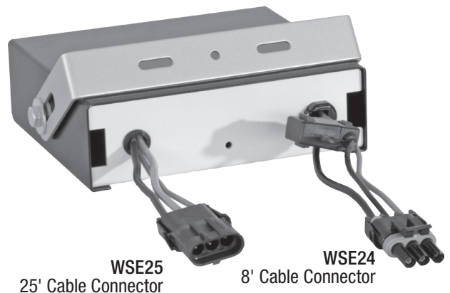
Fig. 5 WSE1 Cab Controller back view
