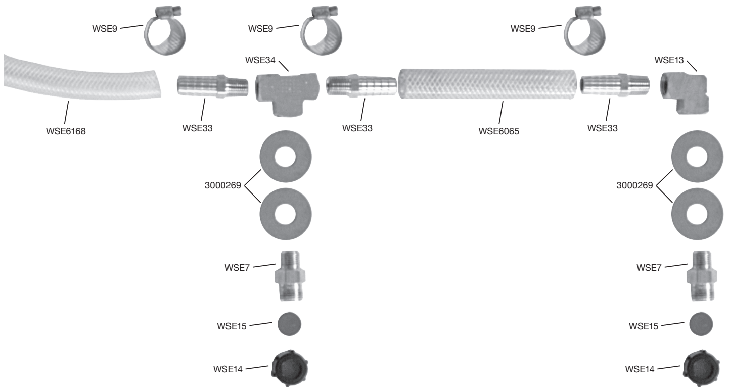
Fig. 7 Nozzle Assembly
