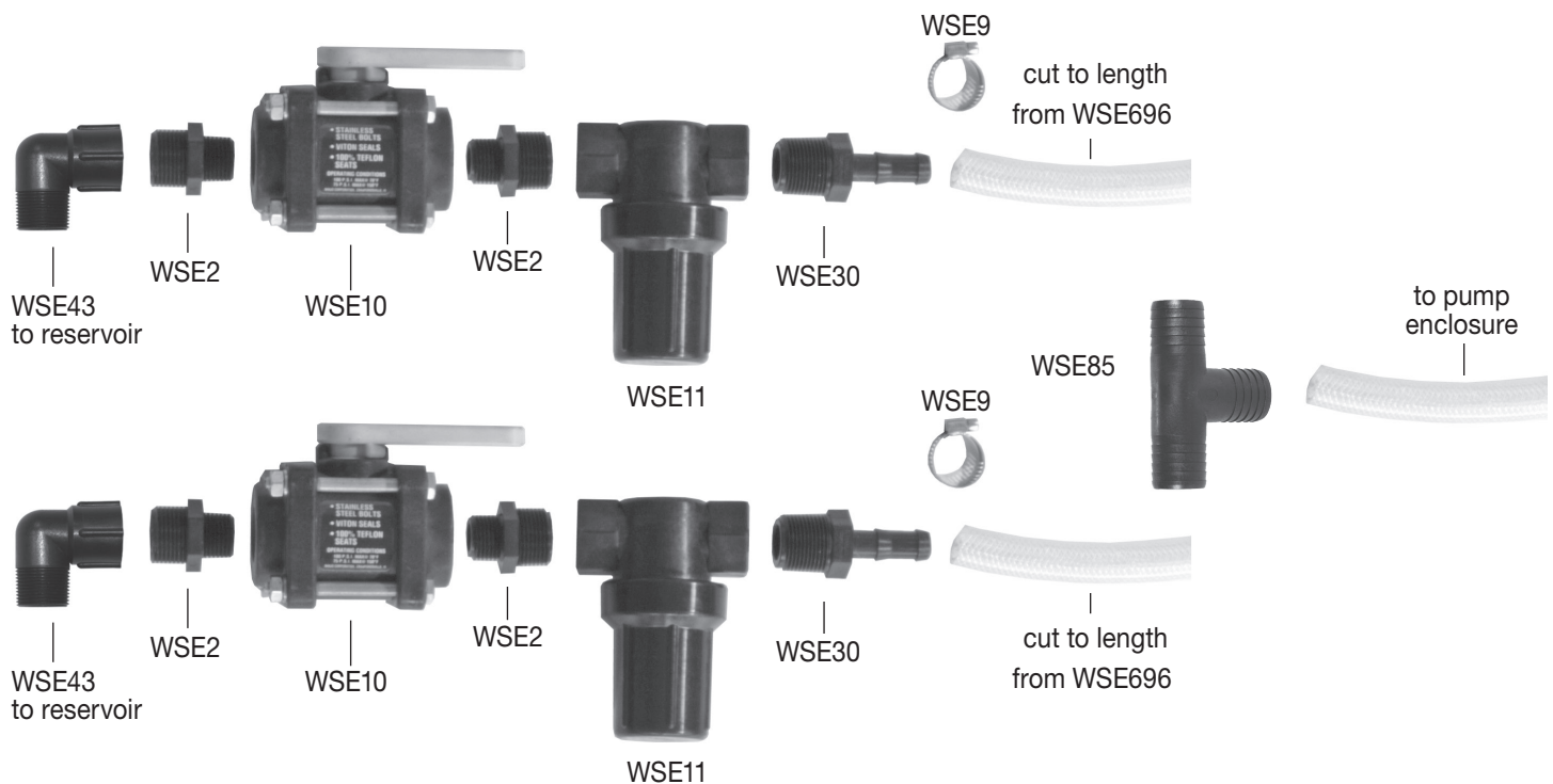
Fig. 7 Filter/Valve Assembly
