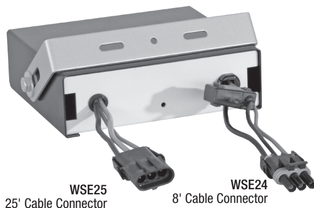
Fig. 4 WSE1 Cab Controller back view
