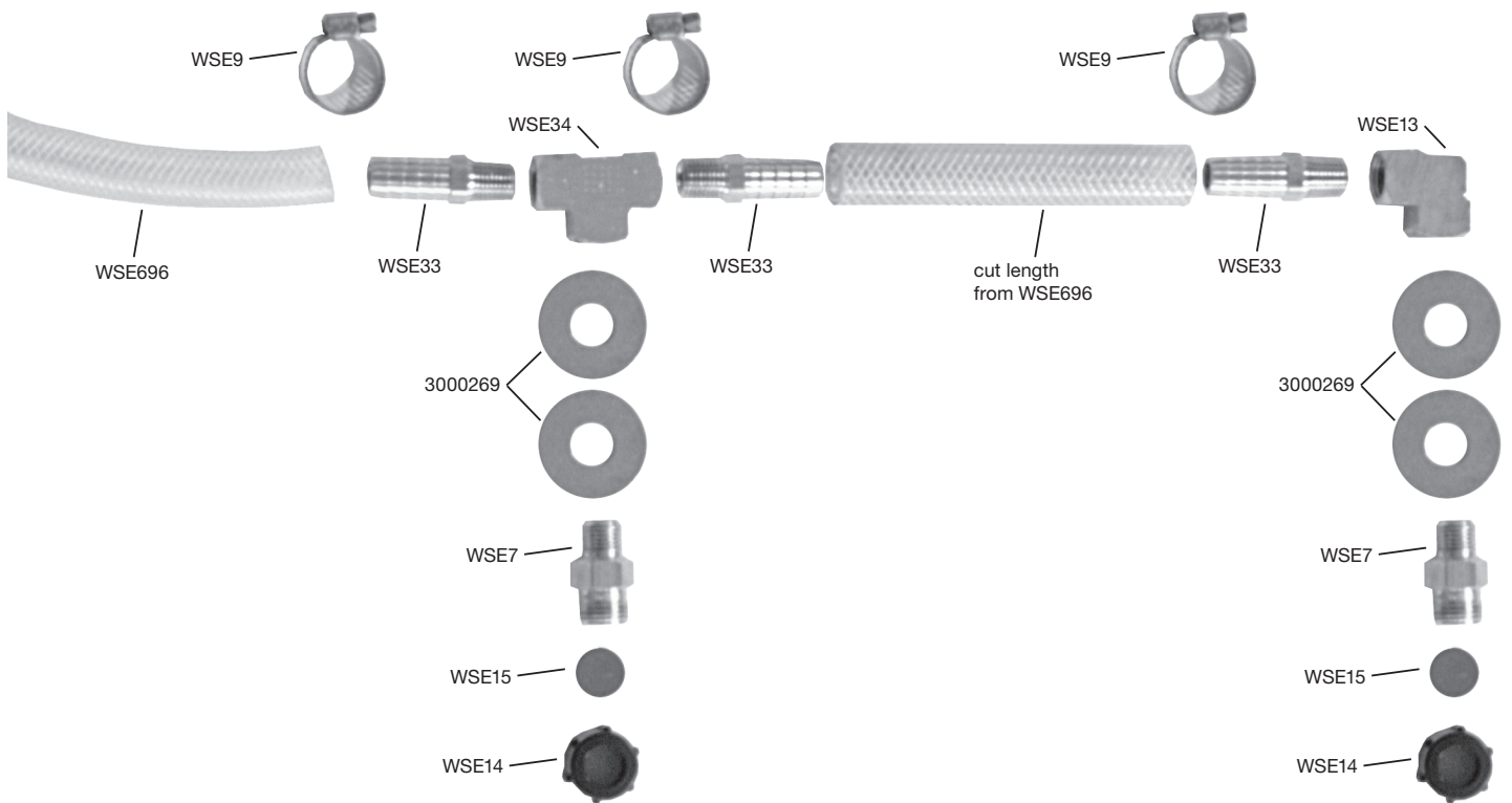
Fig. 9 Nozzle Assembly
