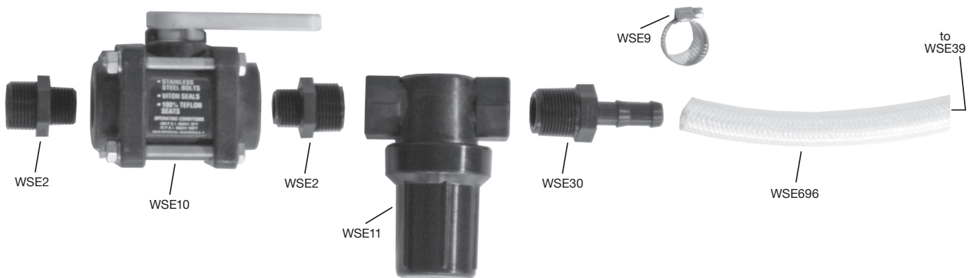
Fig. 10 Filter/Valve Assembly
