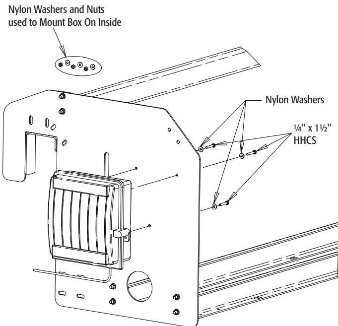
Fig. 3 Control Box
