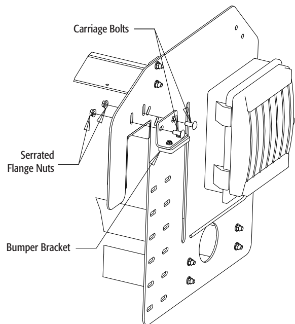
Fig. 4 Bumper Bracket
